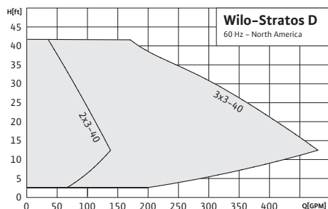
Wilo-Stratos D High Efficiency Circulators
