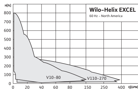
Wilo-Helix EXCEL / EXCEL Complete High Efficiency Multistage Pumps
