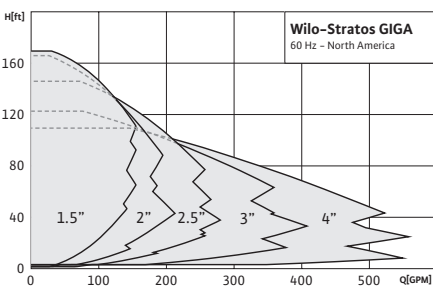
Wilo-Stratos GIGA High Efficiency In-line Pumps
