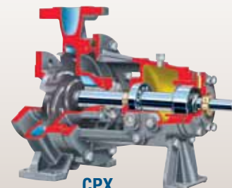
CPX Chemical Process Pump
