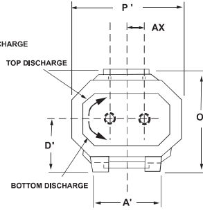
Horizontal configuration (Vertical air flow)
